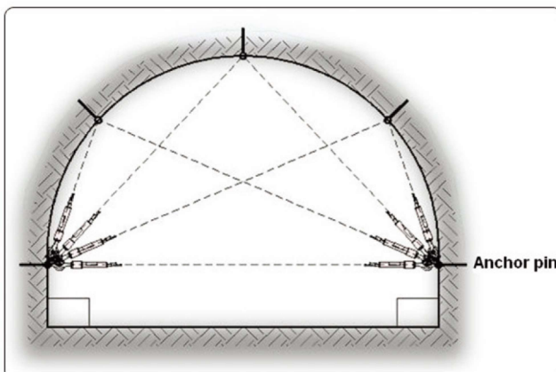
[Measurement drawing of the tunnel convergence displacement]
